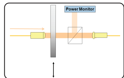
Figure 2. Schematic of multimode attenuator with collimated beam path for homogeneous attenuation and monitoring.
